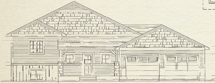
FRONT ELEVATION
