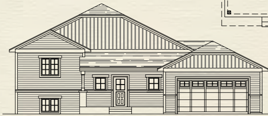
FRONT ELEVATION 2
