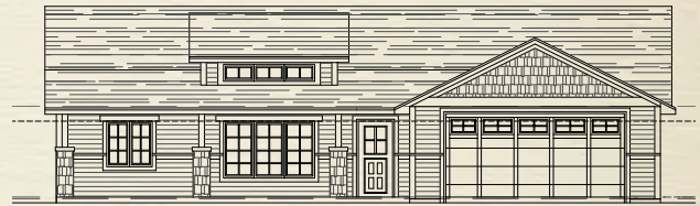
FRONT ELEVATION 1
